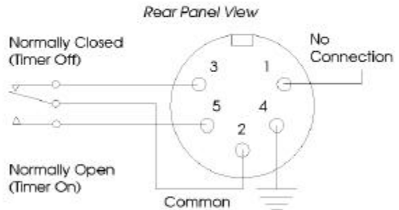
Figure 15 Timer Connections Contacts shown with TIMER OFF
